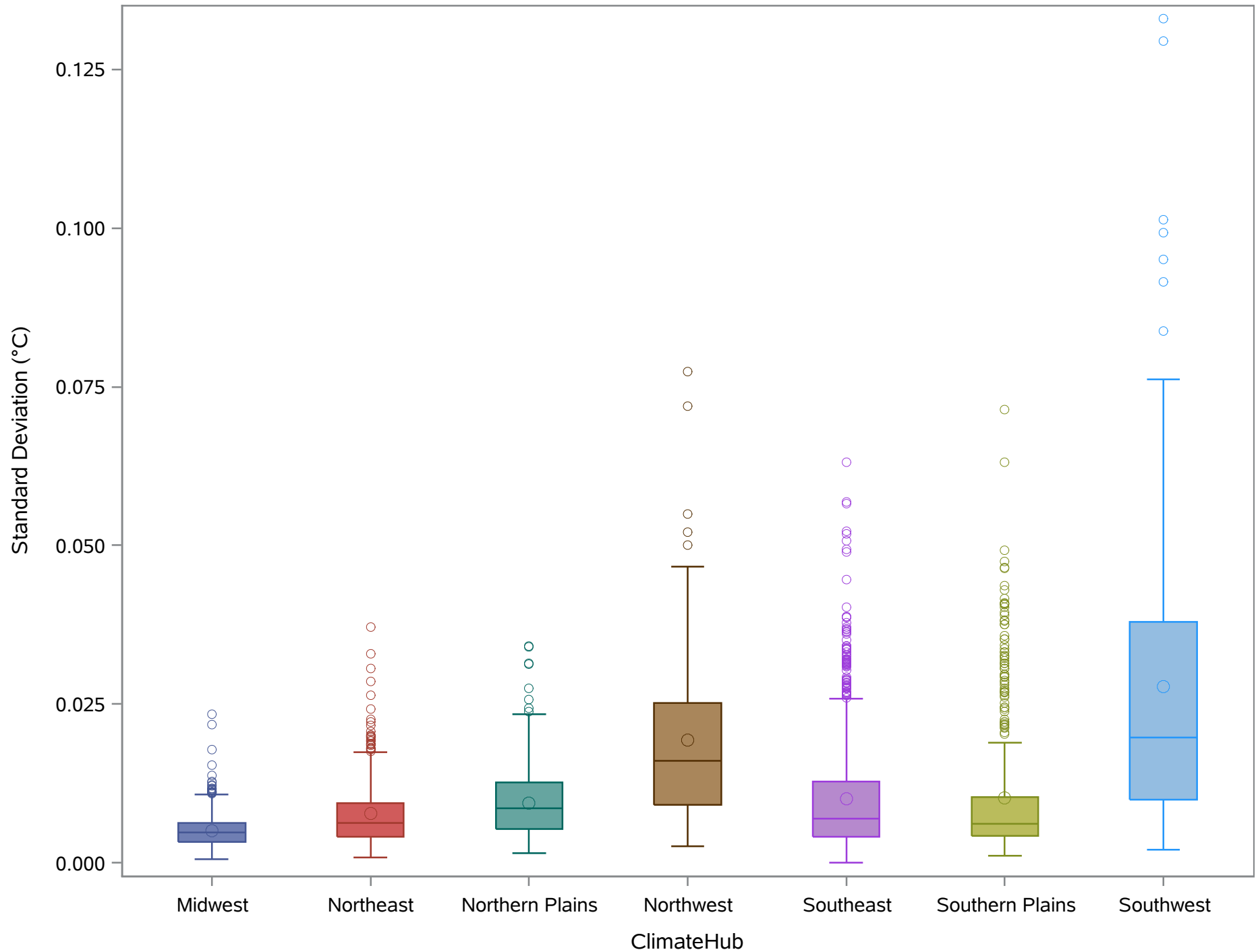
Standard Deviation of Fall Minimum Temperature
