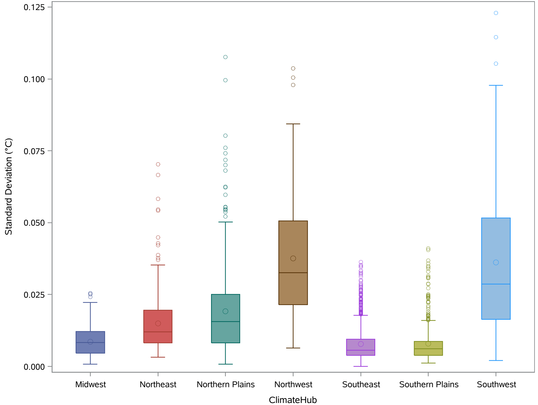
Standard Deviation of Spring Minimum Temperature
