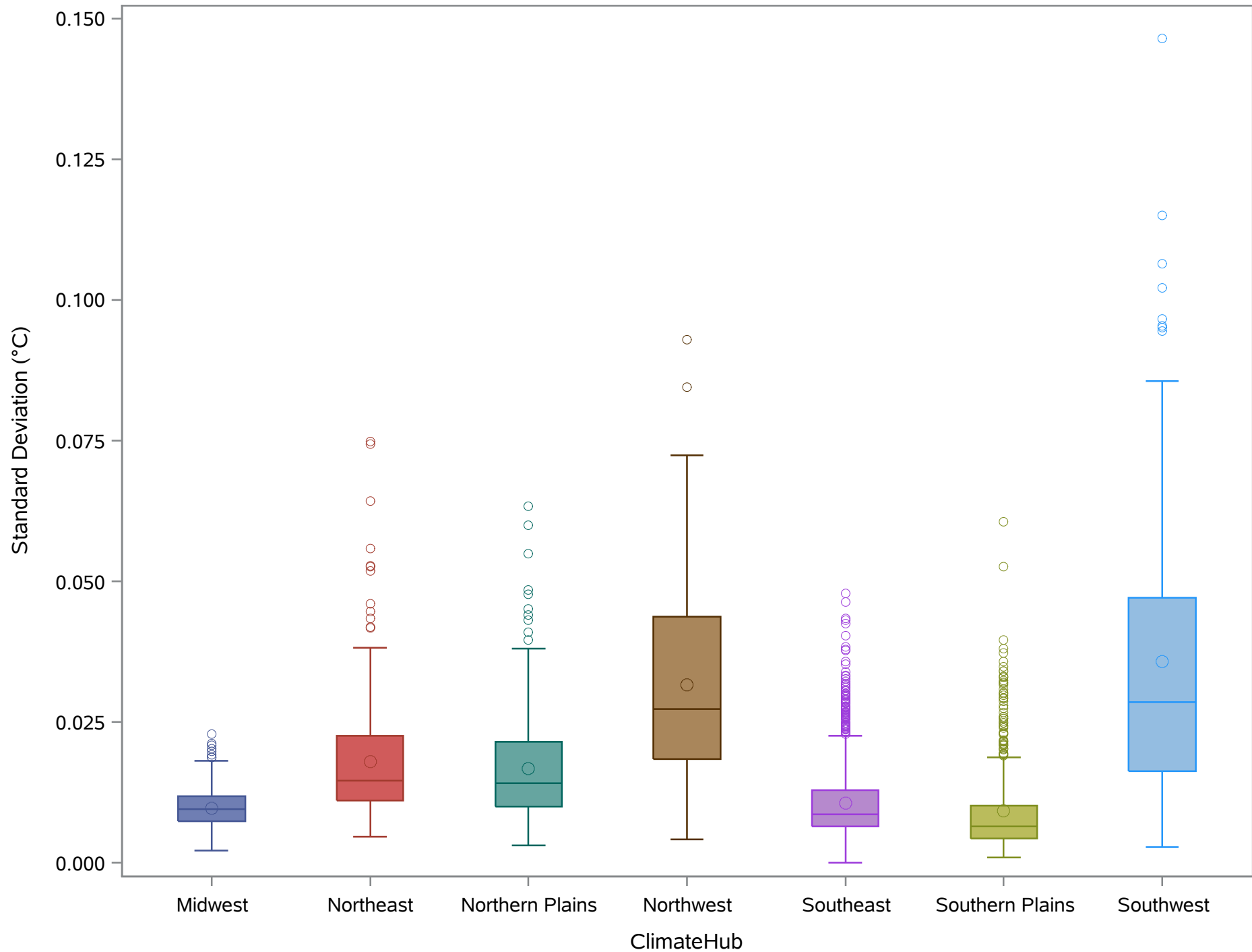
Standard Deviation of Annual Minimum Temperature
