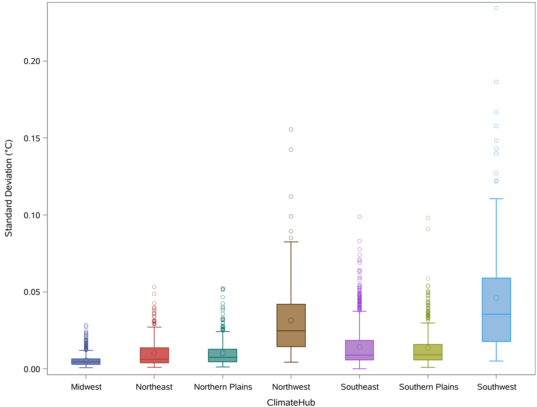
Standard Deviation of Summer Minimum Temperature
