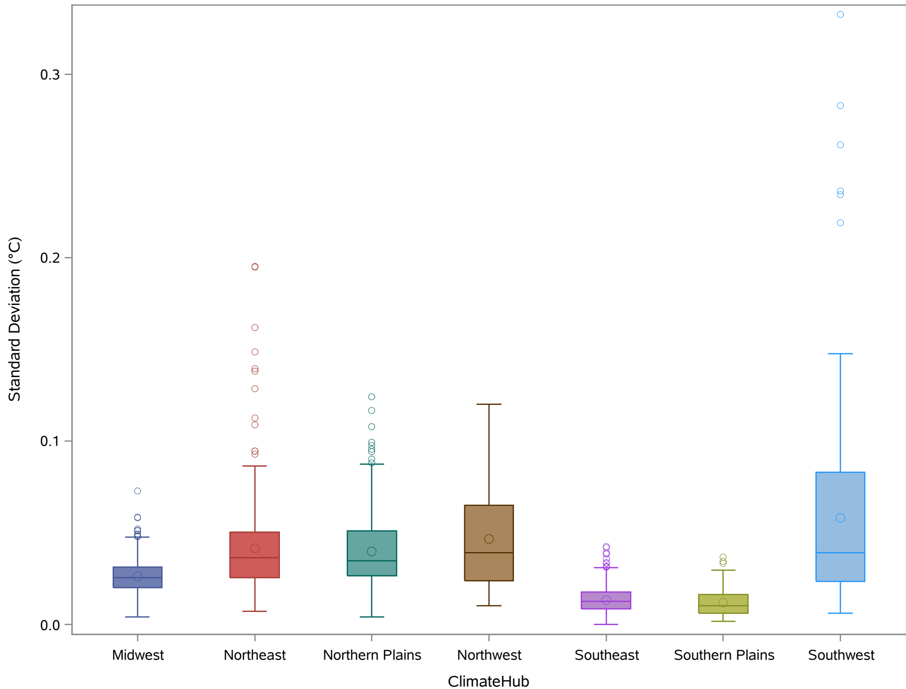
Standard Deviation of Winter Minimum Temperature
